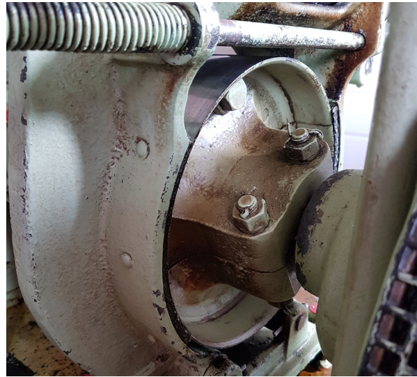
FIGURE 5: Brake pads on lift motor
